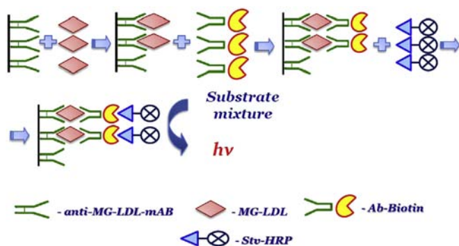
Fig. 2. Scheme of sandwich ELISA for determination of methylglyoxal-modified low density lipoprotein used in this work.
