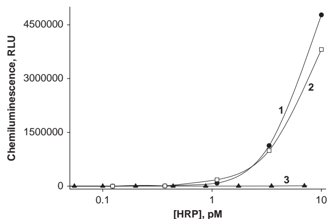
Fig. 1. Dependence of CL intensity produced upon the HRP-catalyzed oxidation of luminol in the presence of (1) PPA, (2) SPTZ and (3) p -iodophenol as primary enhancers on the HRP concentration. The experimental conditions: (1) 100 mM Tris, pH 8.3, containing 1.0 mM luminol, 5.2 mM PPA, 9.3 mM MORPH, and 3.0 mM H_2O_2 ; (2) 80 mM Tris, pH 8.3, containing 0.17 mM luminol, 2.1 mM SPTZ, 8.75 mM MORPH, and 1.75 mM H_2O_2 [12]; (3) 100 mM Tris, pH 8.4, containing 1.0 mM luminol, 1.0 mM 4-iodophenol, 0.5 mM H_2O_2 [13]. Each point represents the mean of duplicates. Vertical bars indicate \pm S.D. about the mean.
