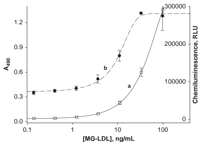
Fig. 3. Calibration curves for determination of MG-LDL by ELISA using (a) chemiluminescent and (b) colorimetric methods to estimate peroxidase activity. Each point represents the mean of duplicates. Vertical bars indicate \pm S.D. about the mean.
